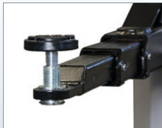
Three-part telescopic lifting arms with double-telescopic lifting plates and twist protection
